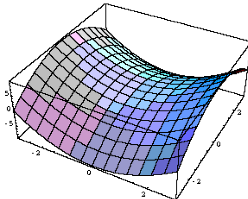
A saddle point
